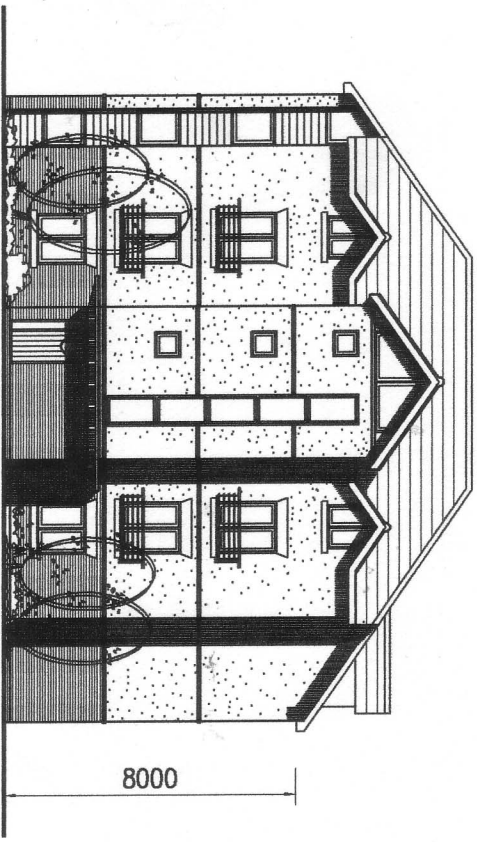
EAST ELEVATION
